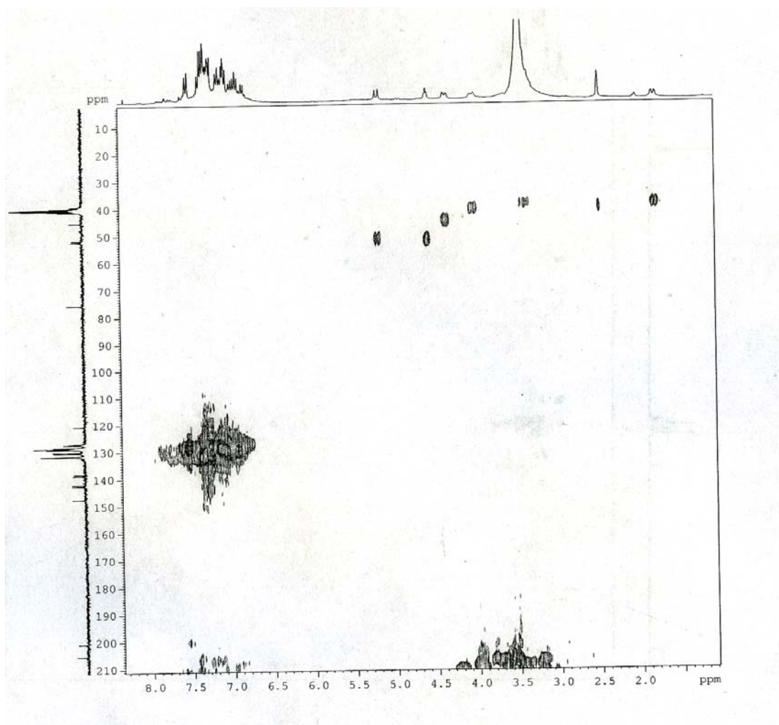
Figure S4. 2D HMQC NMR contour plot of 2 in DMSO-d 6 .
