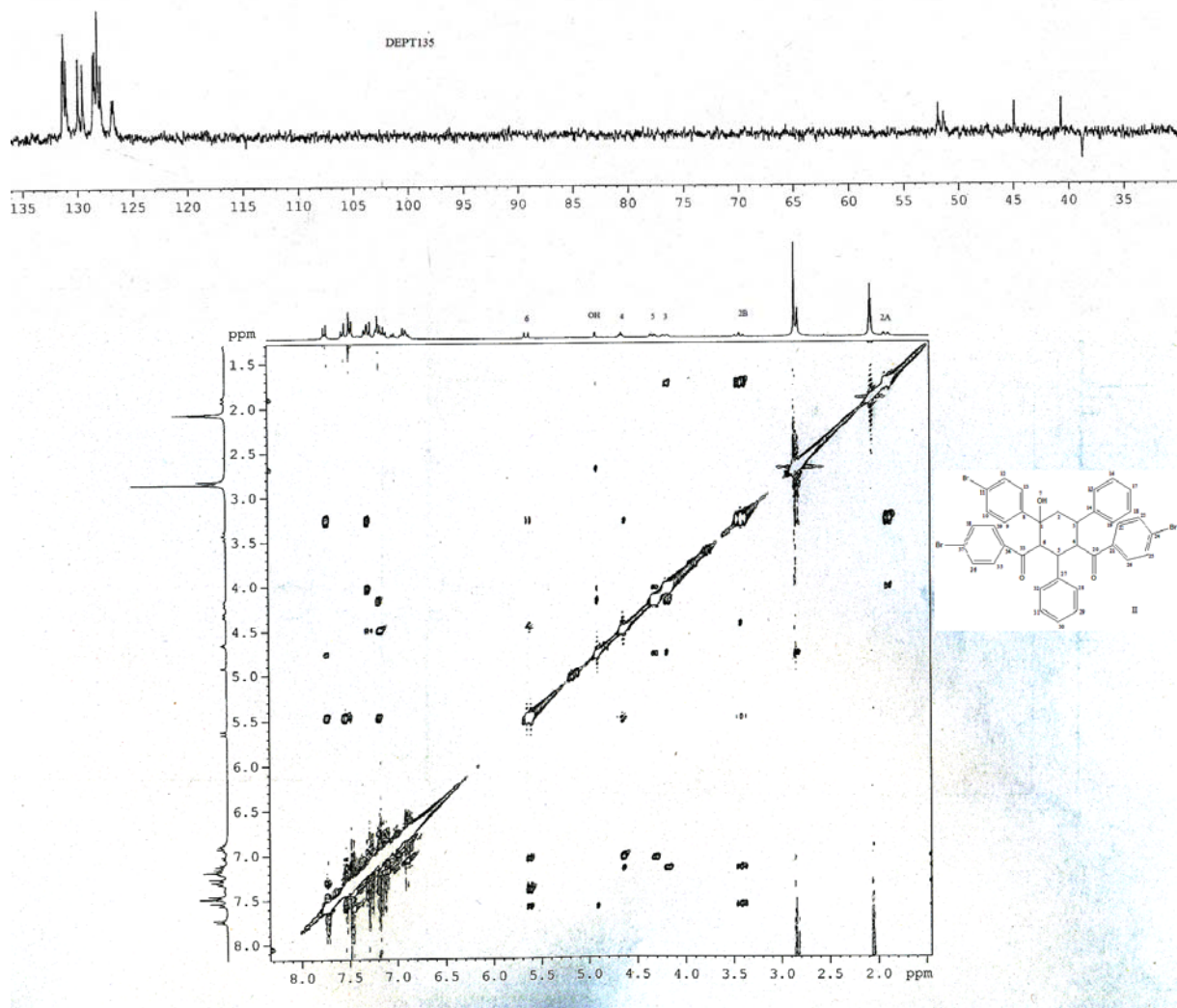
Figure S6. 2D NOESY and DEPT 135 NMR contour plot of 2 in acetone- d_6 .
