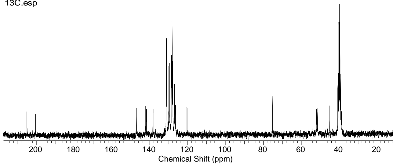
Figure S2. 13 C NMR contour plot of 2 in DMSO-d 6 .
