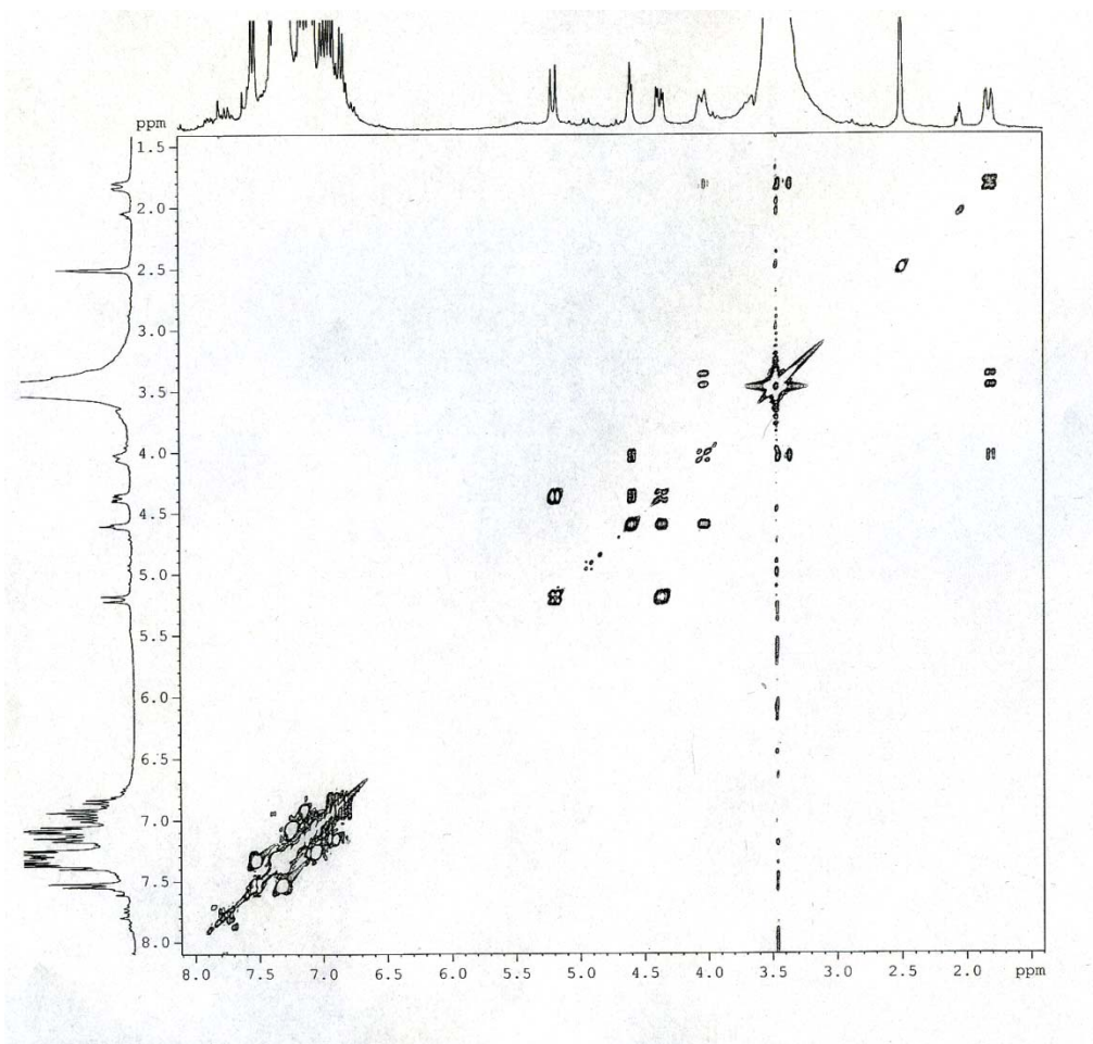
Figure S3. 2D COSY NMR contour plot of 2 in DMSO-d 6 .
