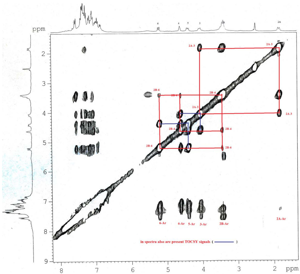
Figure S7. 2D ROESY NMR contour plot of 2 in DMSO- d_6 .
