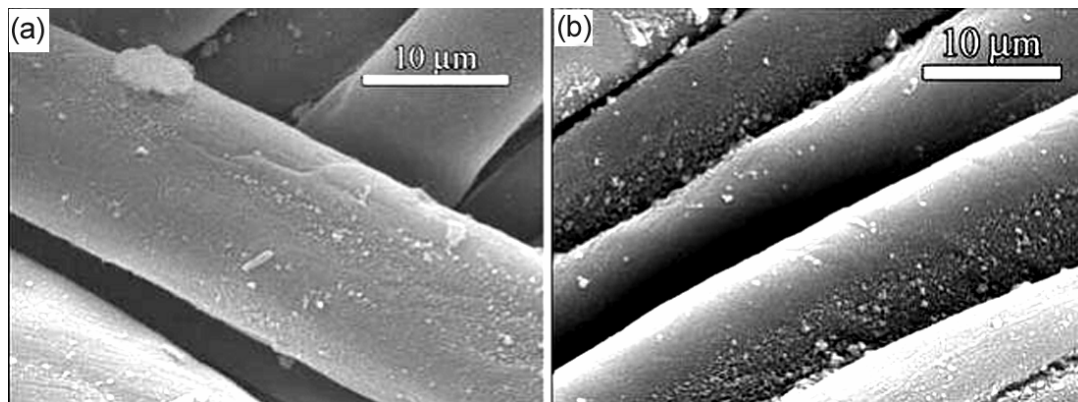
Fig. 4—SEM images of ZnO nanoparticles obtained from Synthesis 1 on (a) polyester/cotton before washing and (b) cotton after washing
