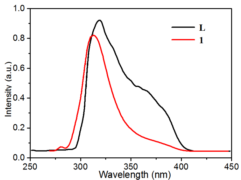
Fig. S2 — Solid-state luminescent spectra of free L ligand and compound 1 at room temperature
