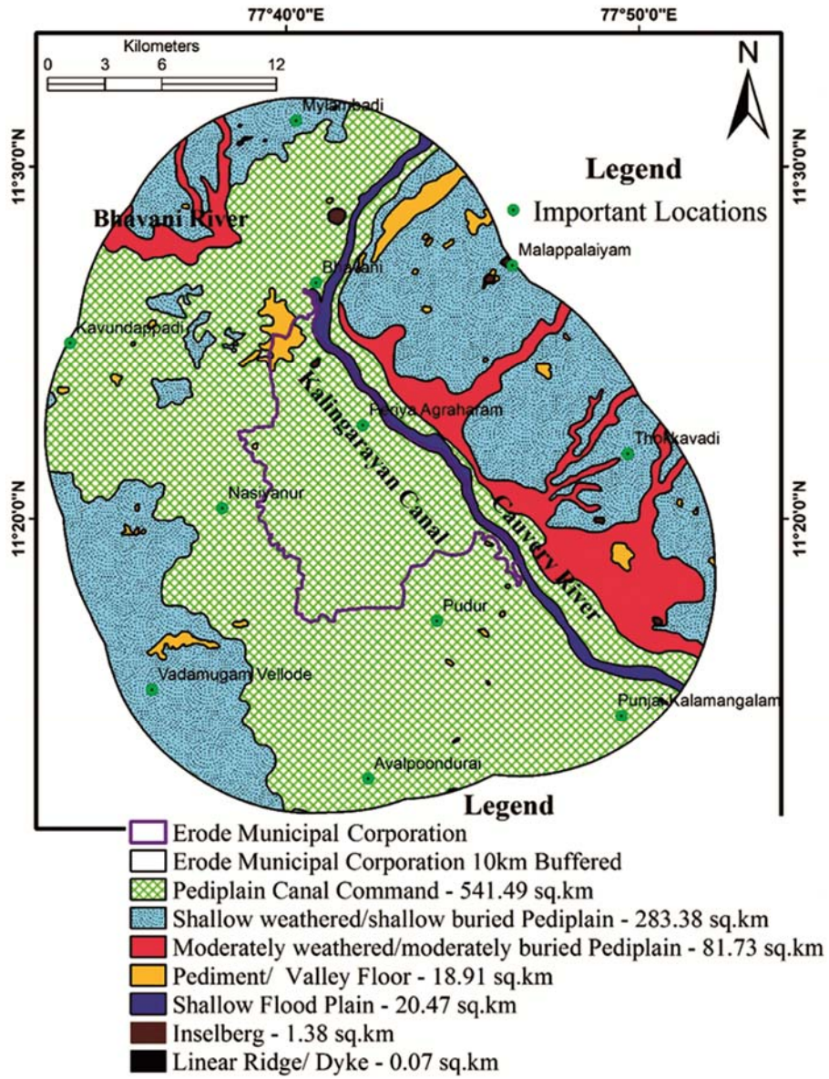
Figure S1 — Spatial map of geomorphology
