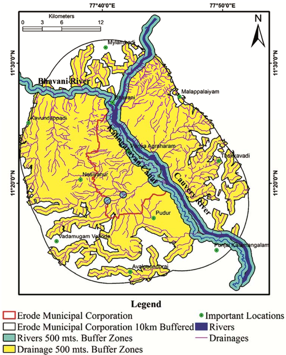
Figure S2 — Spatial map of drainage 500 mts buffer zone
