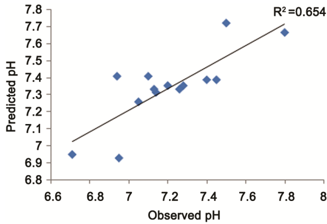
Fig. S1 — Observed vs predicted pH of test set data points
