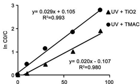
Fig. 6 – Kinetic plot for the photocatalytic degradation of PNP by \text{TiO}_2 and TMAC.
