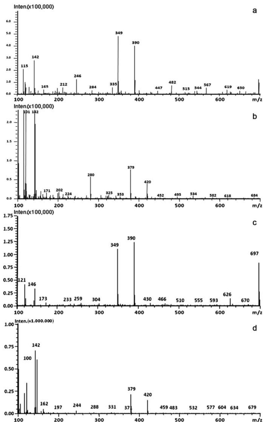
Suppl Fig. 1 (a-d)—Electron mass spectra of CPT (M+H) + at m/z 349 and methoxy CPT at m/z 379.12 in callus samples (a & b) and fruit samples (c & d).
